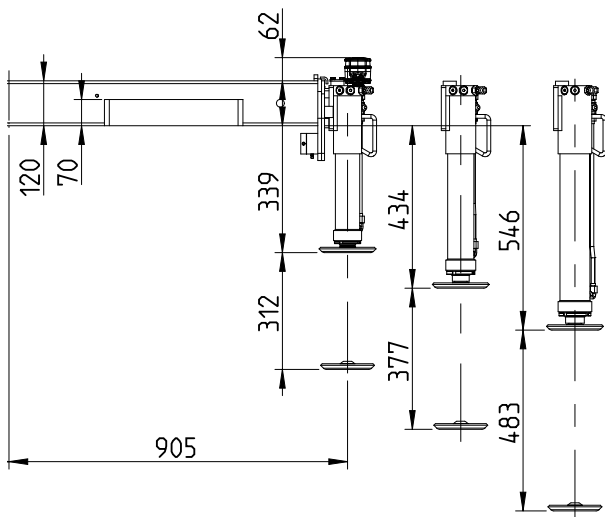
FIXED STABILIZER WITH TILTING DEVICE
