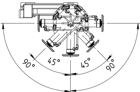
STABILIZER WITH TILTING DEVICE PARKING POSITION
