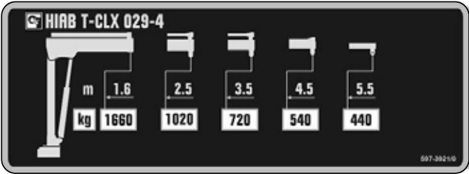
Capacity plate HIAB T-HIDUO 029-4
