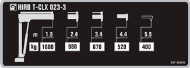
Capacity plate HIAB T-CLX 023-3
